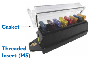
00580K 8 Way Axial Kit
